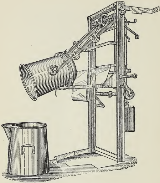
FIG. 23.—Weber's Elevator, Final Position.
